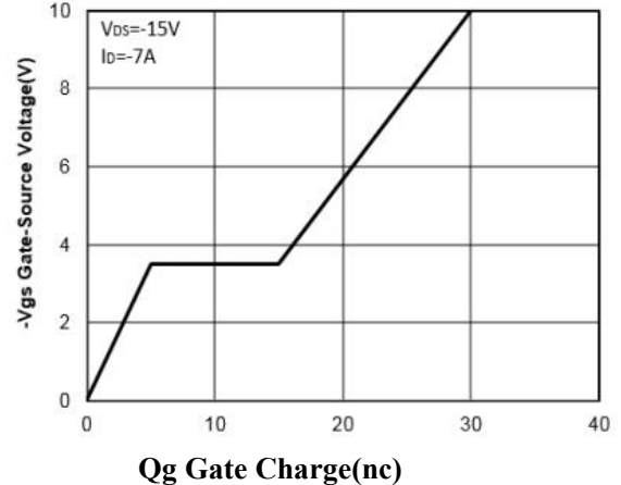
Figure 6: Gate-Charge Characteristics
