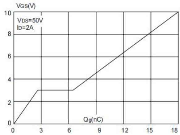
Figure 6: Gate-Charge Characteristics
