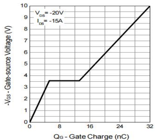
Figure 6: Gate-Charge Characteristics
