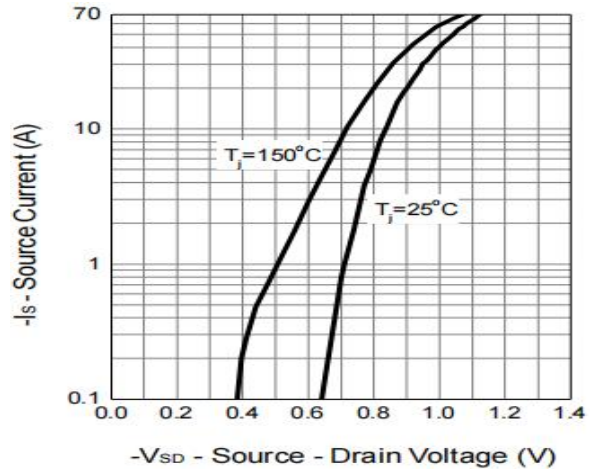
Figure 2: Diode Characteristics
