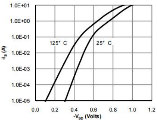
Figure 7: Diode Characteristics
