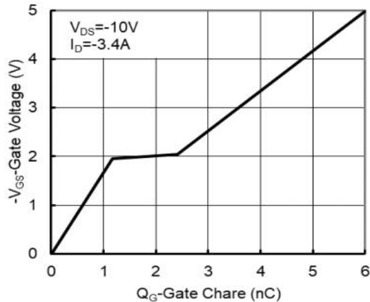
Figure 6: Gate-Charge Characteristics
