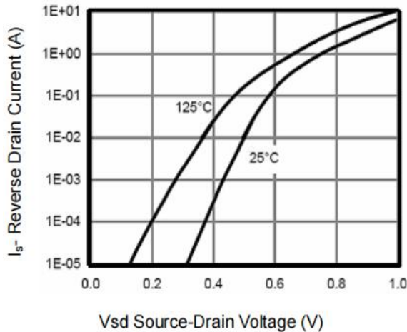
Figure 9: Diode Characteristics
