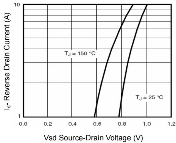
Figure 7: Diode Characteristics
