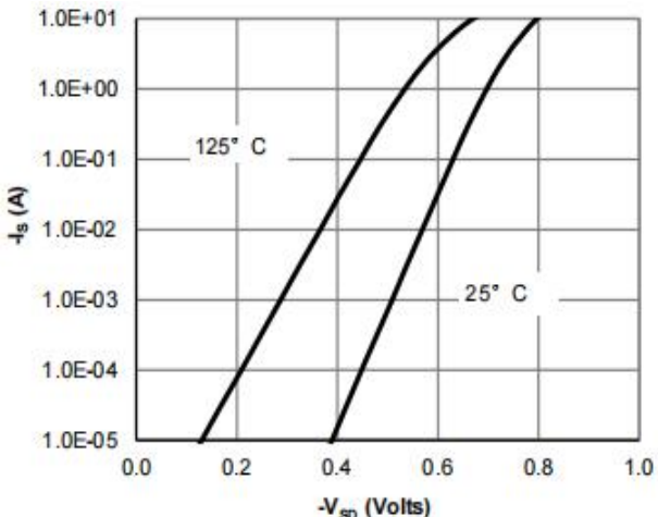
Figure 3: Diode Characteristics
